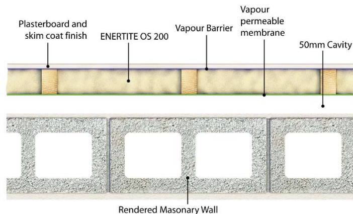
Figure 2: Masonry Wall – Dry Lining
